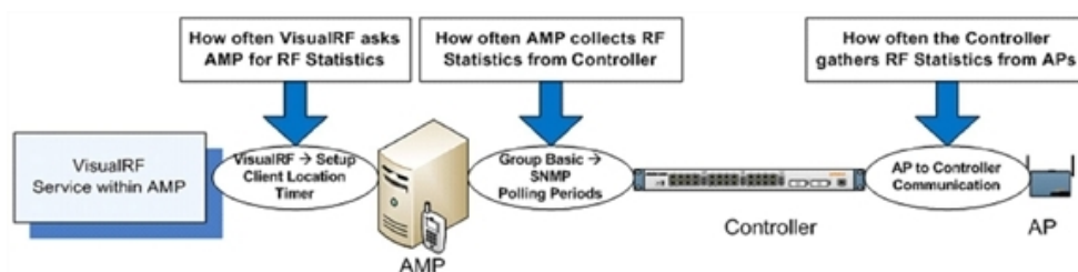
Figure 224 Timing Factors Impacting Location Accuracy
